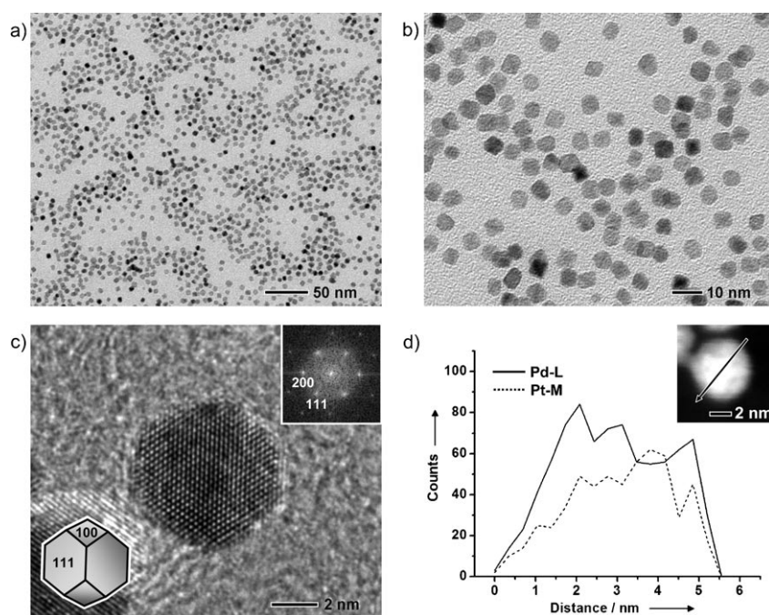
Figure 4. a,b) TEM images of Pd–Pt alloy nanocrystals synthesized by co-reducing \text{Na}_2\text{PdCl}_4 and \text{K}_2\text{PtCl}_4 with EG as a reducing agent. The reaction was conducted at 110^\circ\text{C} for 5 h, with the molar ratio of \text{Na}_2\text{PdCl}_4 to \text{K}_2\text{PtCl}_4 at 1:1. c) HRTEM image of a single truncated octahedron shown in (a) recorded along the [011] zone axis. The insets show the corresponding FT pattern (upper right) and the geometrical model of the truncated octahedron (lower left). d) Compositional line profiles of Pd and Pt from the truncated octahedron recorded along the line shown in the HAADF-STEM image (inset).
